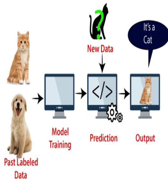
Figure 7: SVM classification
