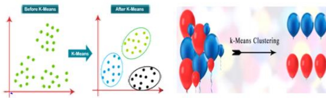
Figure 5: Finding Clusters
