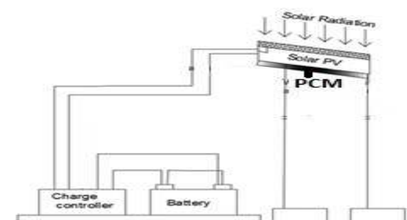
Figure 4: Schematic diagram of solar still
