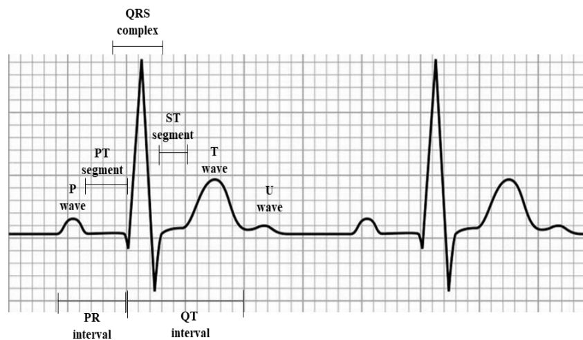
Figure 2: Normal ECG
