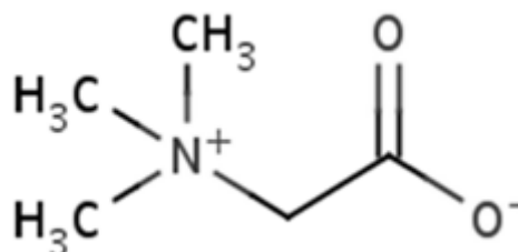
Figure 5: Glycine Betaine
