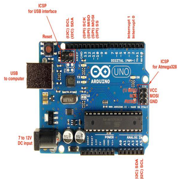
Figure 1: Arduino Uno R3
