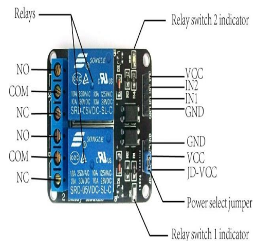
Figure 3: 2-channel relay
