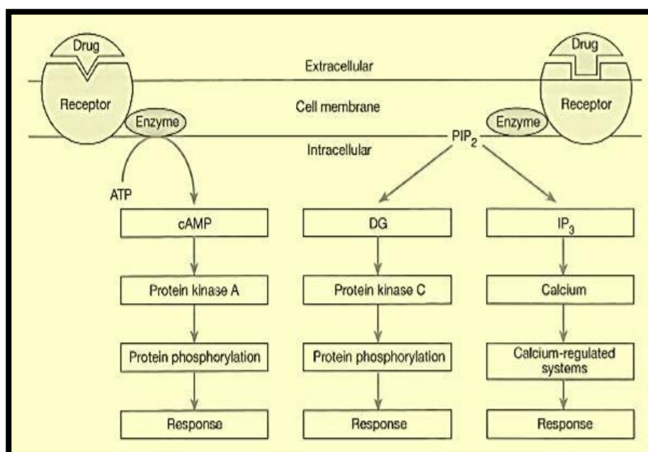
Figure 1: An illustration of the two kinds of second messenger systems that mediate how medications acting on G-protein coupled receptors affect the body.
