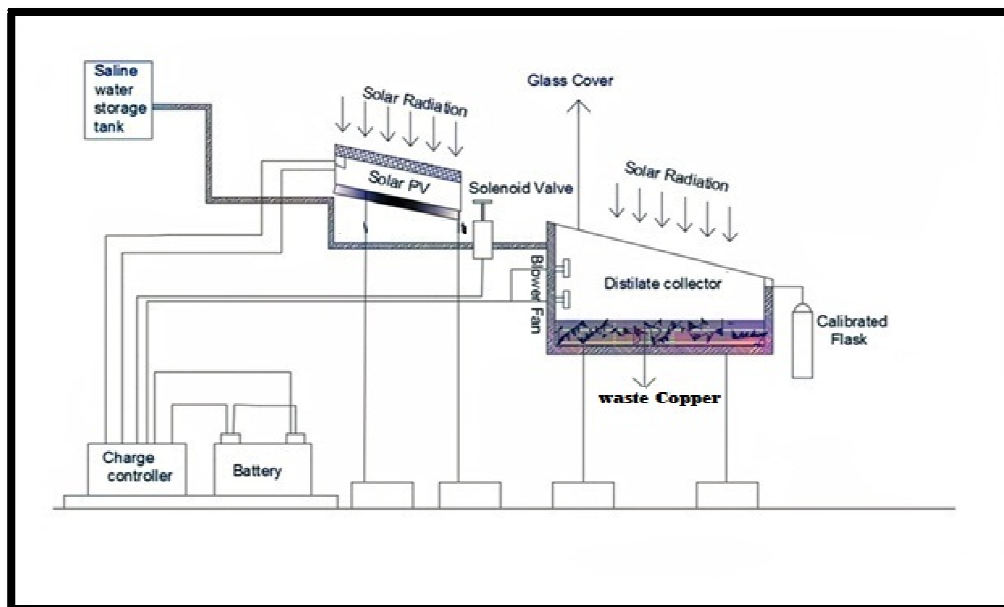
Fig 4: Schematic diagram of solar still
