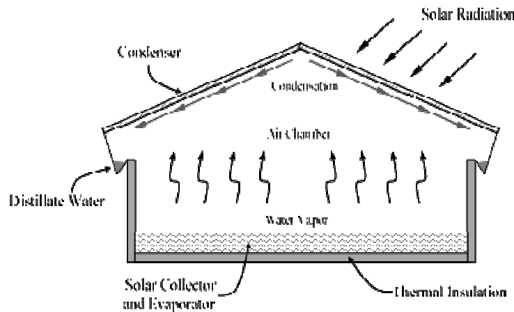
Figure 3: Dual slope solar still
