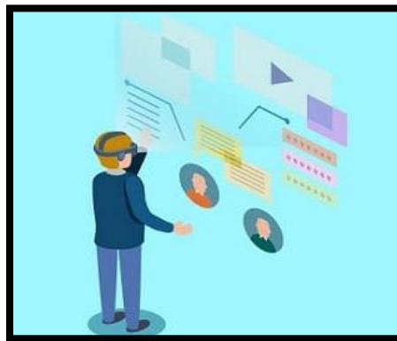
Figure 8: Augmented Reality
