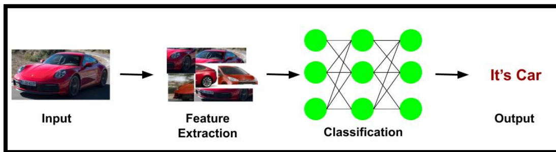
Figure 2: Machine learning
