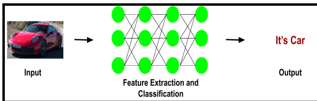
Figure 3: Deep Learning
